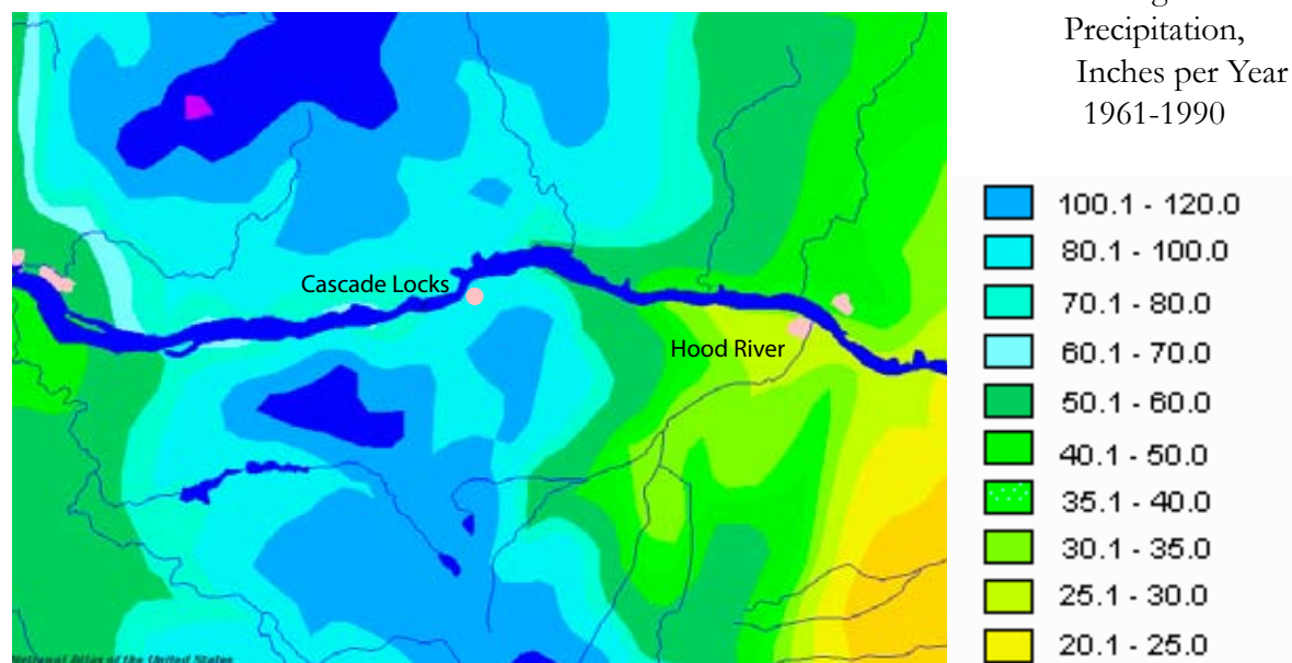
Figure 2. Climate zones within the Columbia Gorge, from 70 to 80 inches of rain per year at Cascade Locks to less than 30 inches per year at Hood River. Created from National Atlas. Opposite page: project area map, courtesy of HAER. Columbia River Highway Project 1981
