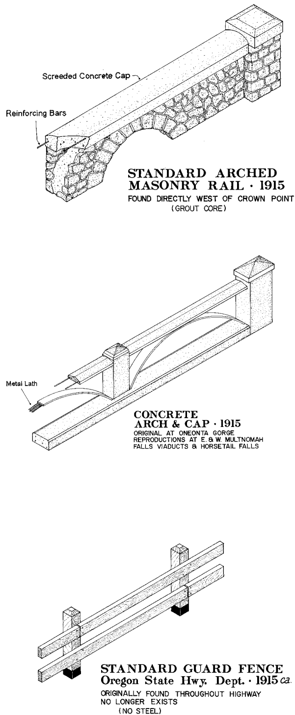
Figure 7. Guard rail types. Courtesy of HAER.
